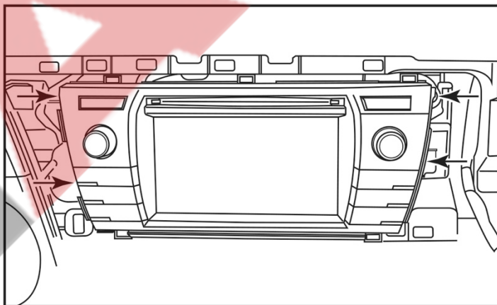
Unfasten two (2) bolts two on each side of the radio unit.
